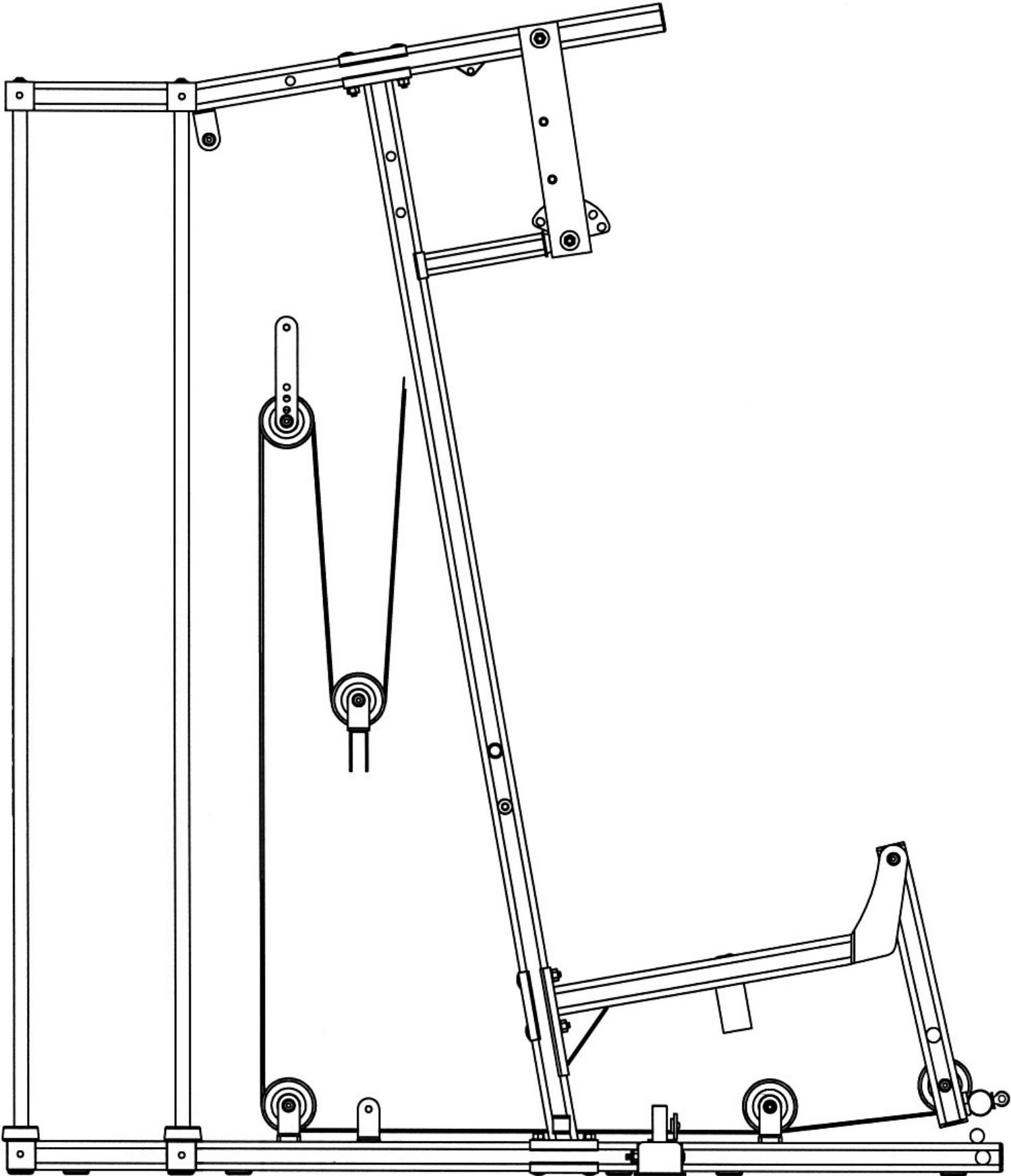
Lower Cable Loop Diagram
