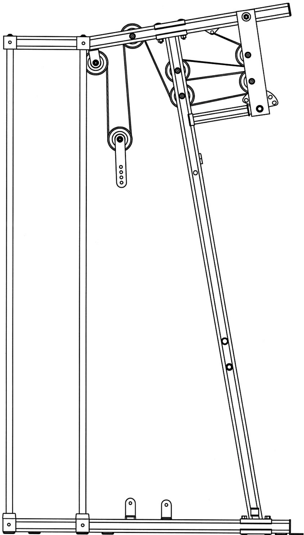
Front Press Cable Loop Diagram
